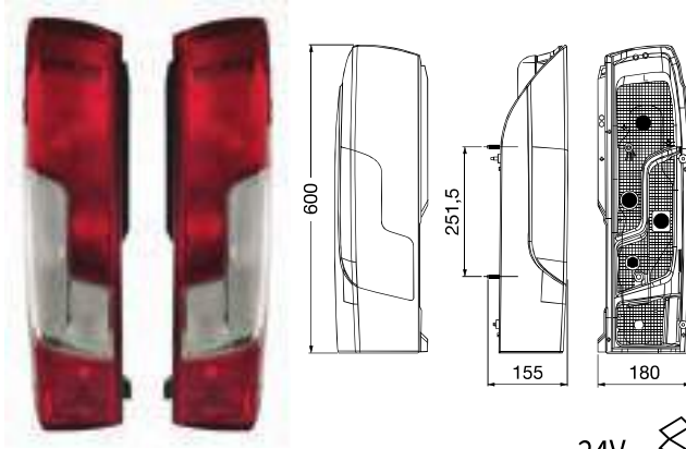
Rear Combination Lamp (without Socket) Arka Kombinasyon Lambası (Soketsiz)
